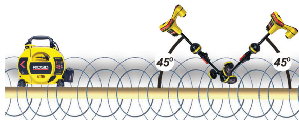
Figur 5 – 45°-luttest
